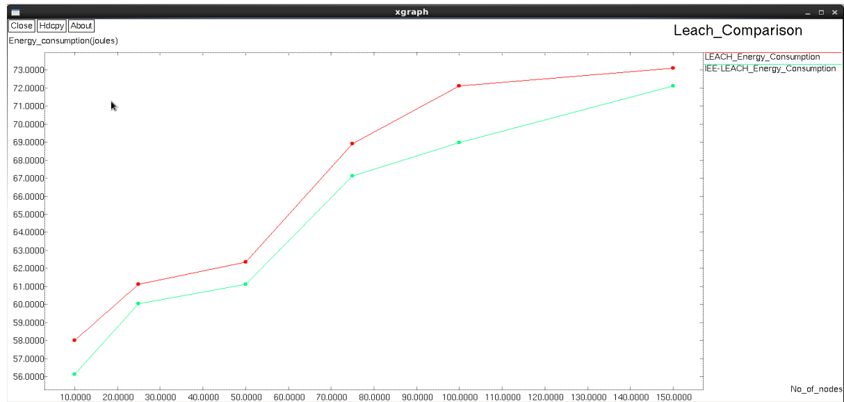
Figure 6: Energy consumption of Leach and IEE-LEACH Protocol
